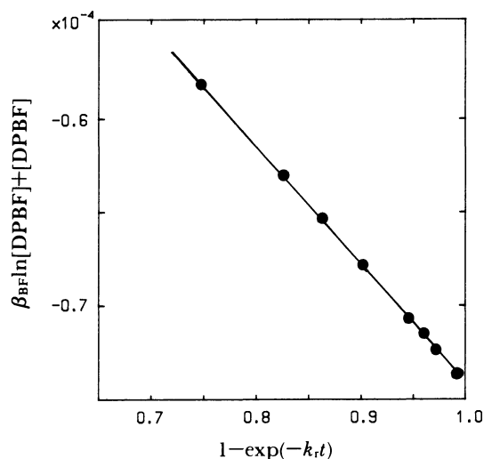
Fig. 3. Kinetic treatment for oxygenation of DPBF with ^1\text{O}_2 regenerated by the thermal decomposition of \text{DPFO}_2 at 45^\circ\text{C} . (The values for k_r of 1.59 \times 10^{-2} and for \beta_{\text{BF}} of 1.99 \times 10^{-5} are used in Eq. 18.) [MB]: 5 \mu\text{M} ; [DPF]: 68 \mu\text{M} ; [DPBF]: 49 \mu\text{M} .
